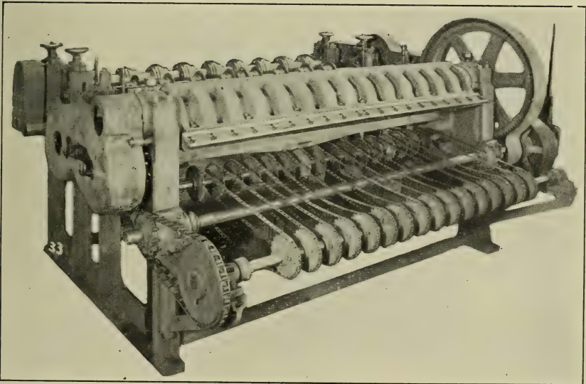
FIG. 136.—Shingle Cutter—Rear View.
